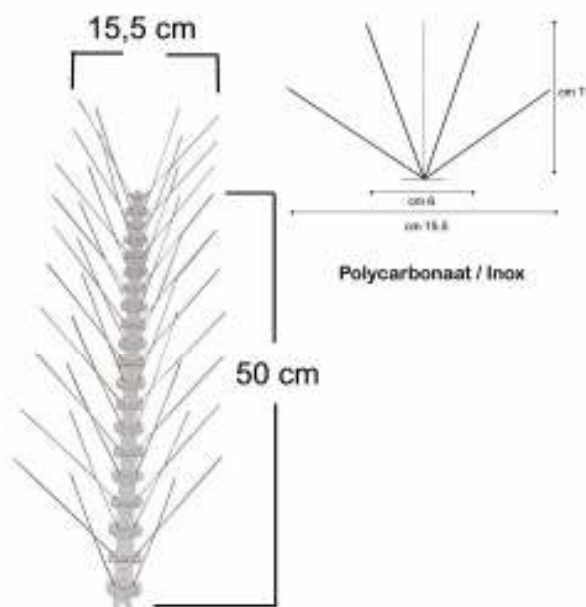
Scare Spikes model 311
